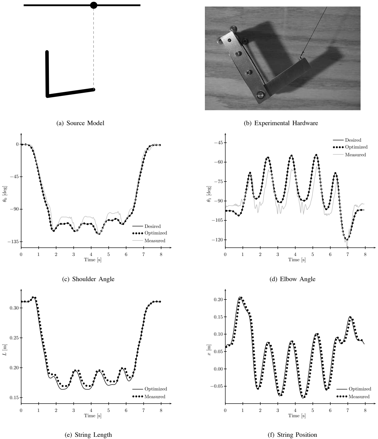
Fig. 2. Animation-based source models (a) and experimental hardware setup (b). Plots of the desired, optimized, and measured shoulder (c) and elbow (d) angles as well as the corresponding system inputs (e,f). The optimized trajectories match the desired trajectories well.
