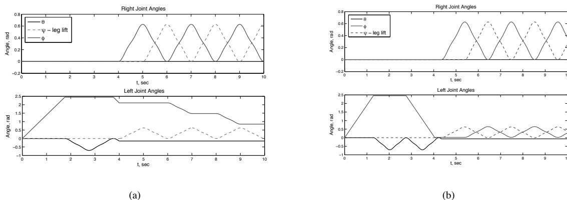
Fig. 3. Plots of the joint angles for left and right limbs during the execution of the original 3(a) and optimized 3(b) MDL strings.
