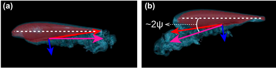
Figure 6. Snapshots of forward swimming (a) and backward swimming (b) simulated black ghost knifefish.
